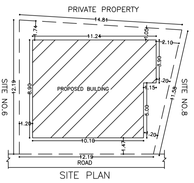
SITE PLAN
