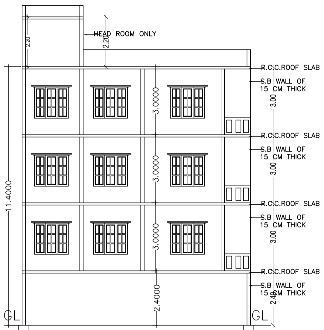
SECTION @ AA
